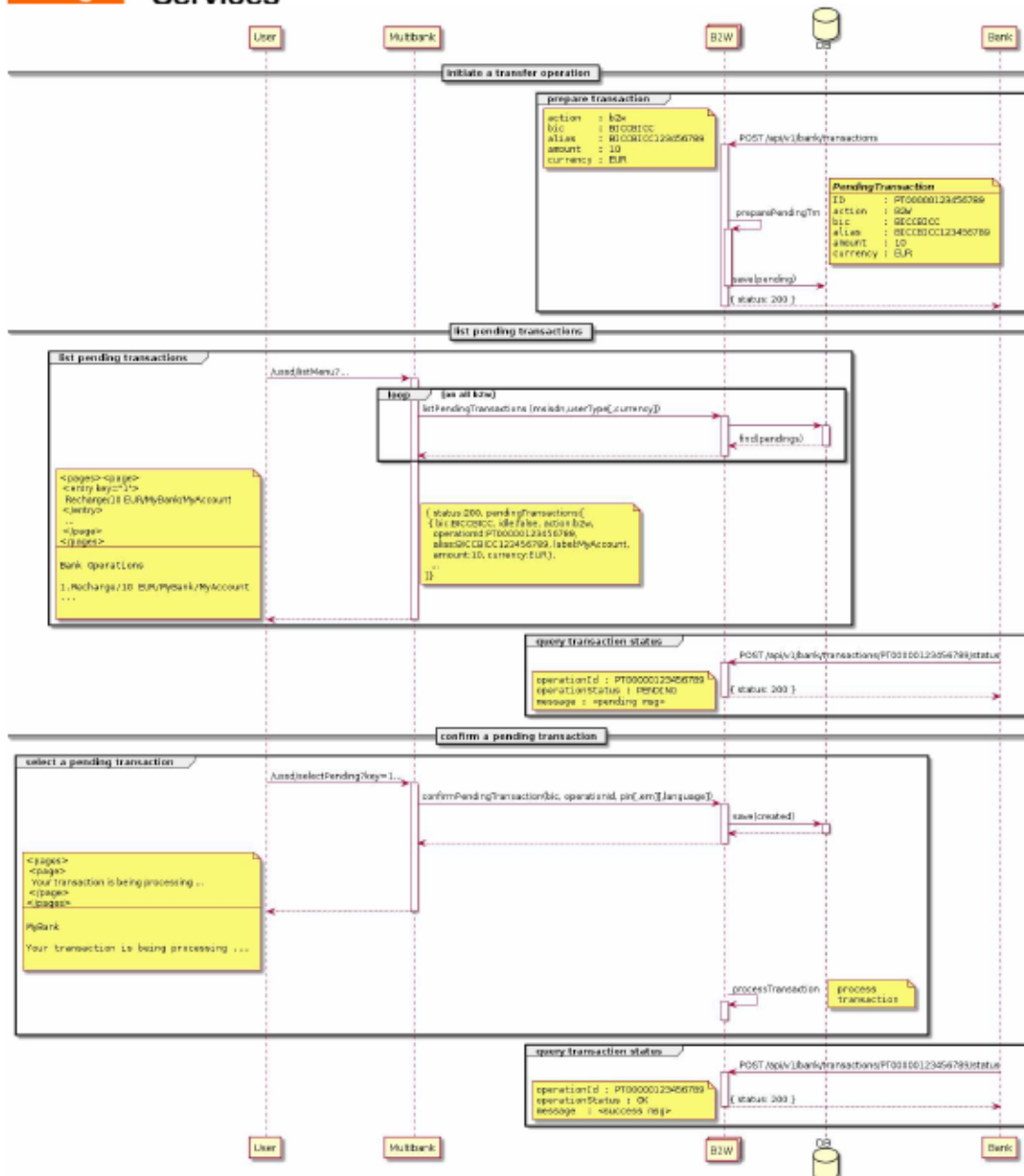
bank initiated transaction sequence diagram
